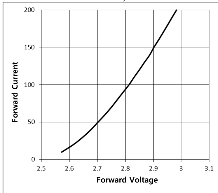
Fig 3. Forward Voltage vs. Forward Current, T_j = 25^\circ\text{C}
