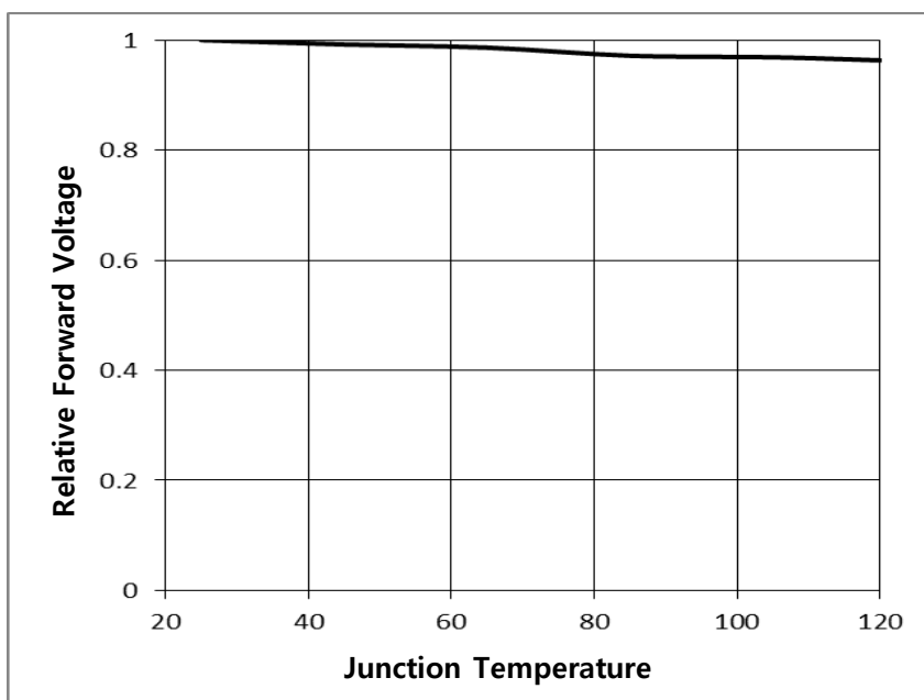
Fig 7. Junction Temperature vs. Relative Forward Voltage, I_F=65\text{mA}
