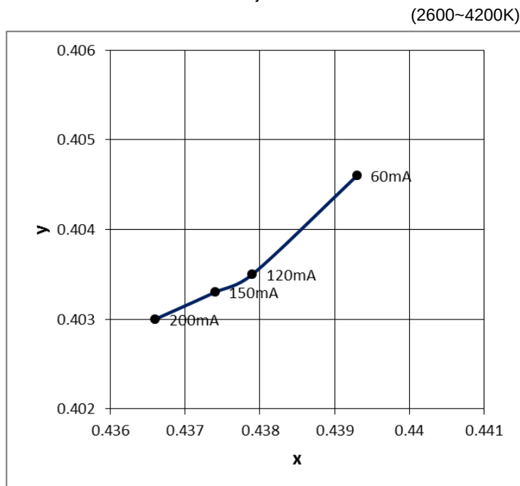
Fig 5. Forward Current vs. CIE X,Y Shift, T_j = 25^\circ\text{C}
