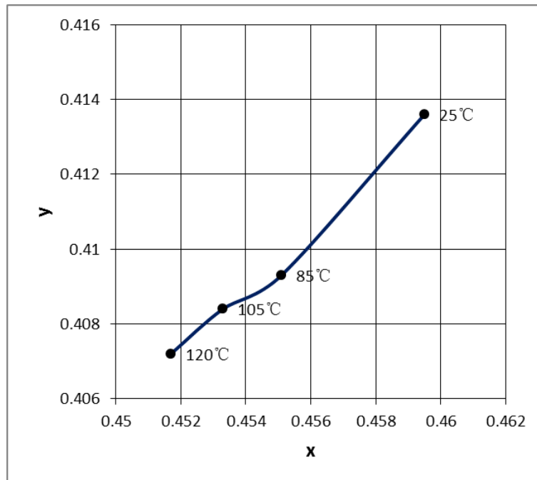
Fig 8. Chromaticity Coordinate vs. Junction Temperature, I_F=65\text{mA} (2600~4200K)
